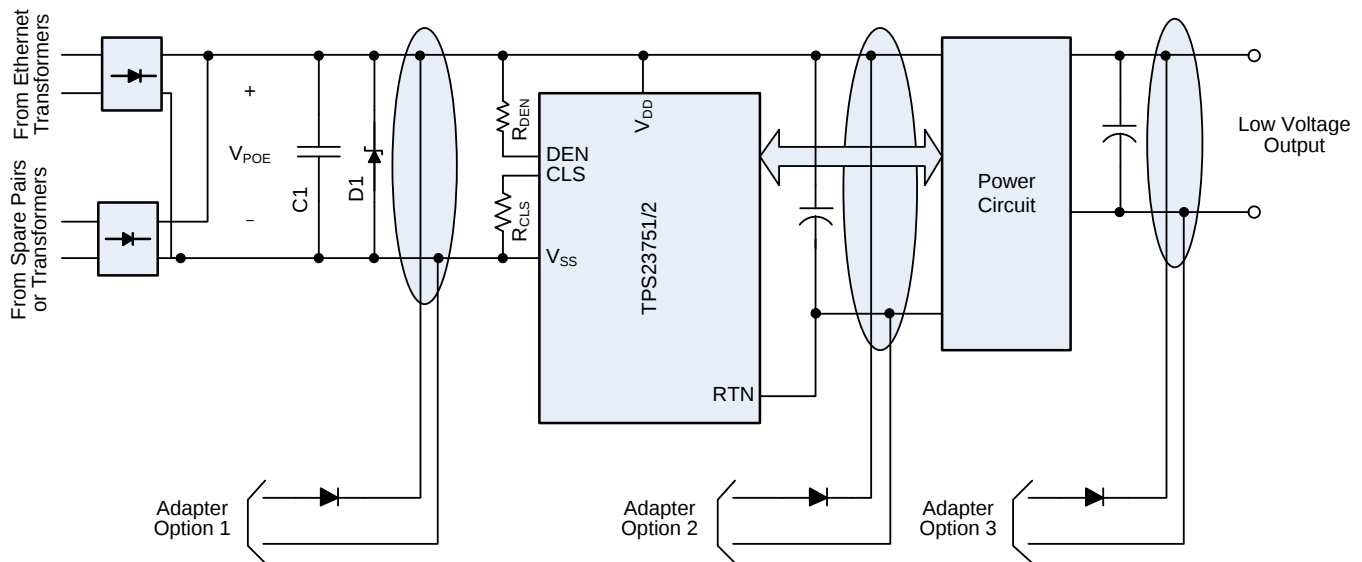
Figure 31. ORing Configurations
