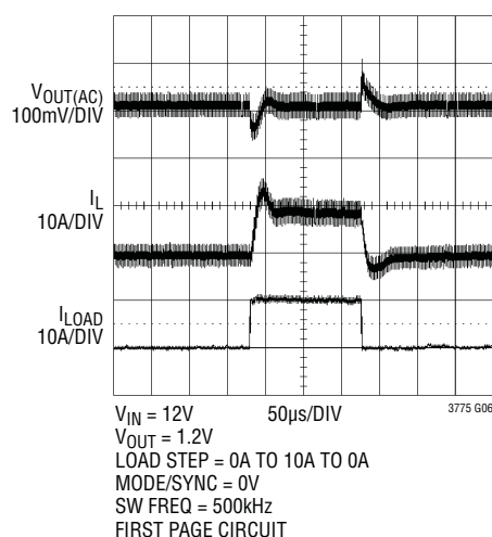
Load Step in Forced Continuous Mode
