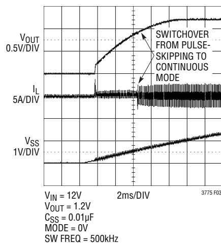
Figure 3. Typical Start-Up Wavform for a Buck Converter Using the LTC3775
