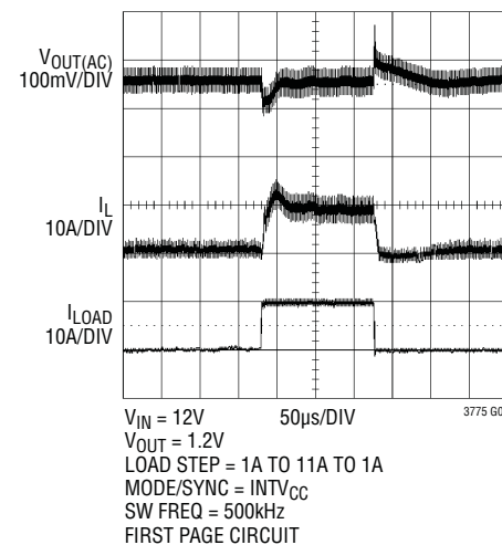
Load Step in Pulse-Skipping Mode
