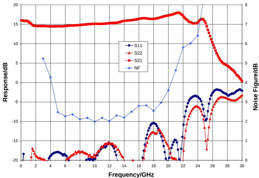
Broadband Performance, V_{dd} = 5\text{ V} , I_{dd} = 80\text{ mA} , T_A = 25^\circ\text{C}
