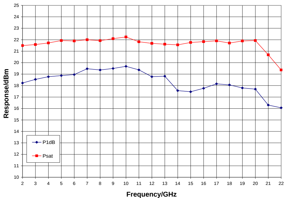
Output Power, V_{dd} = 5\text{ V} , T_A = 25^\circ\text{C}
