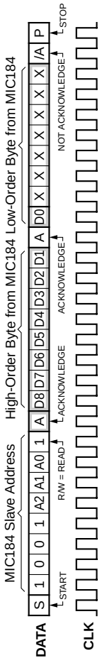
Figure 4. READ_WORD Protocol
