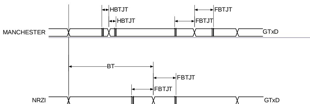
Figure 12: GSC Transmit Timings (Internal Baud Rate Generator)
