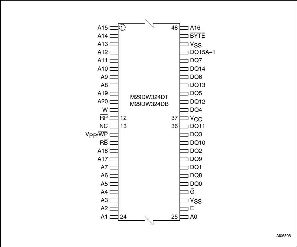
Figure 3. TSOP Connections
