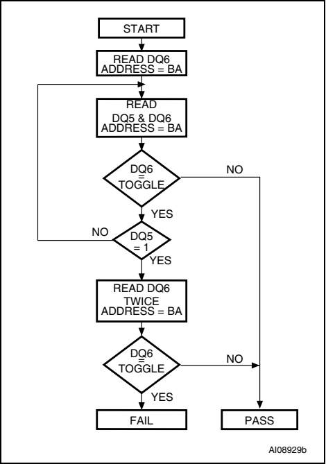
Figure 8. Toggle Flowchart
