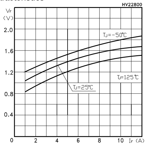
Figure 18: Emitter-Collector Diode Characteristics
