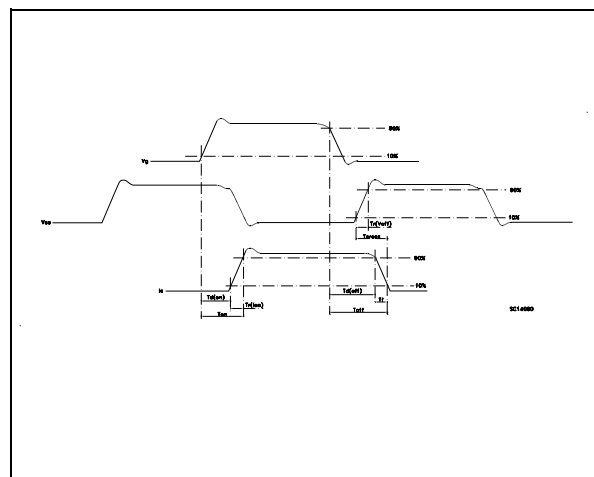
Figure 21: Switching Waveforms
