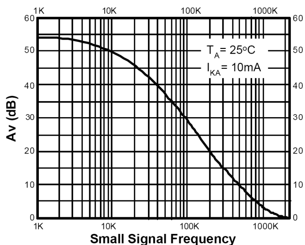
Small Signal Voltage Gain vs. Frequency
