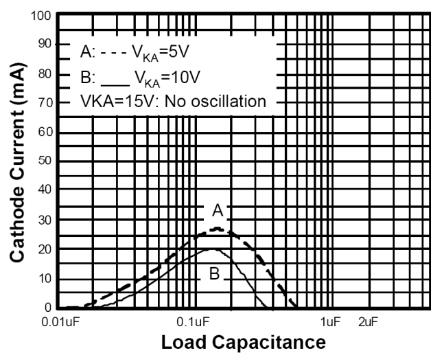
Stability Boundary Conditions vs. Load Capacitance
