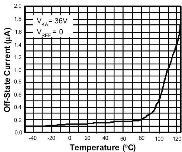
Off-State Current vs. Temperature
