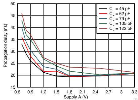
图 6-7. Typical Propagation Delay of Low-to-High (A to B) vs Load Capacitance
