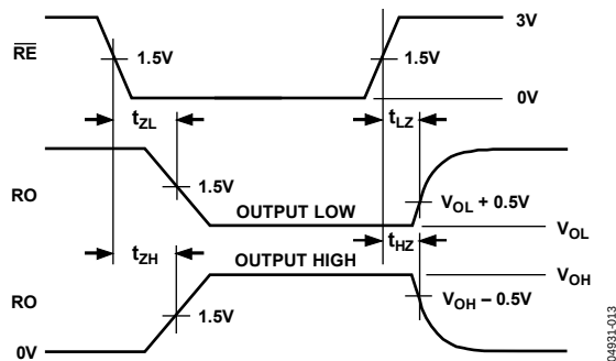
Figure 27. Receiver Enable/Disable Timing
