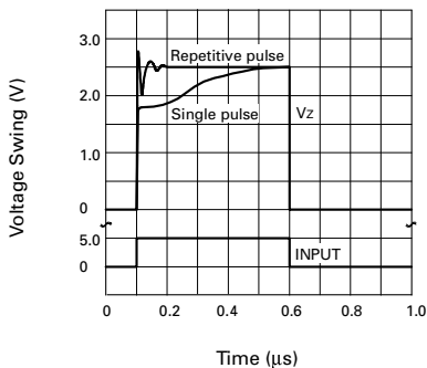
Pulse Response
