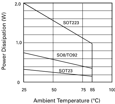
Power Dissipation Derating
