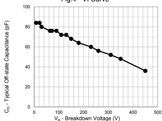
Fig.6 - Typical Off-state Capacitance
