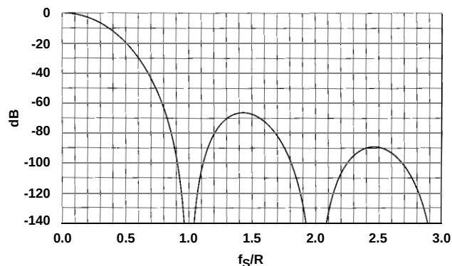
FIGURE 15. 5TH ORDER ( N = 5 ) CIC RESPONSE ( R = DECIMATION FACTOR, f_s/R = 1 is CIC OUTPUT RATE)
