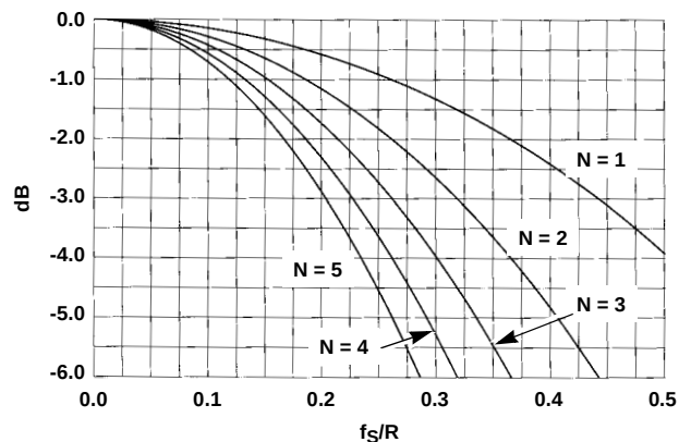
FIGURE 13. CIC PASSBAND ROLLOFF ( N = # OF STAGES, R = DECIMATION FACTOR, f_s/R = 1 is CIC OUTPUT RATE)
