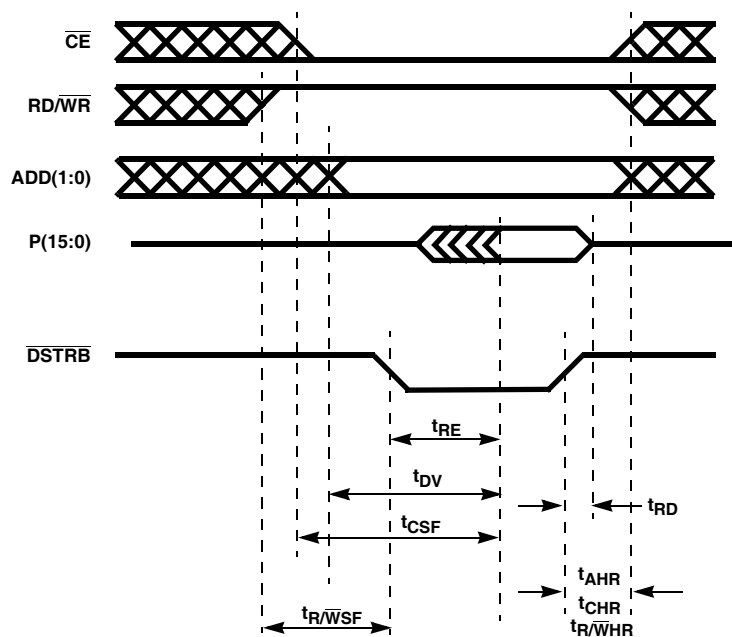
FIGURE 10. MICROPROCESSOR READ TIMING ( \mu\text{P} MODE = 1)
