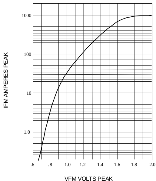
Fig. 1-TYPICAL INSTANTANEOUS FORWARD CHARACTERISTICS AT T_j = 25^\circ\text{C}
