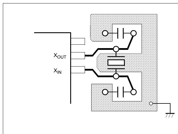
Figure 18-2 Layout of Oscillator PCB circuit
