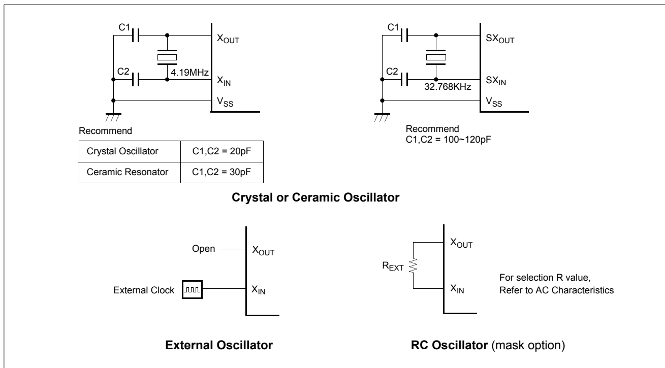
Figure 18-1 Oscillation Circuit
