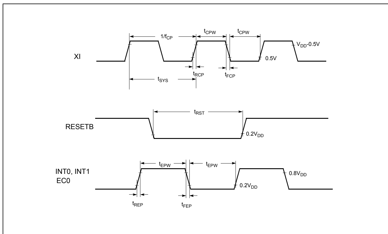
Figure 7-1 Timing Chart
