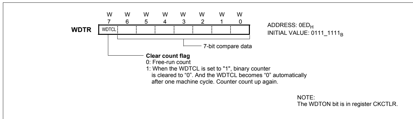
Figure 11-2 WDT: Watchdog Timer Data Register
