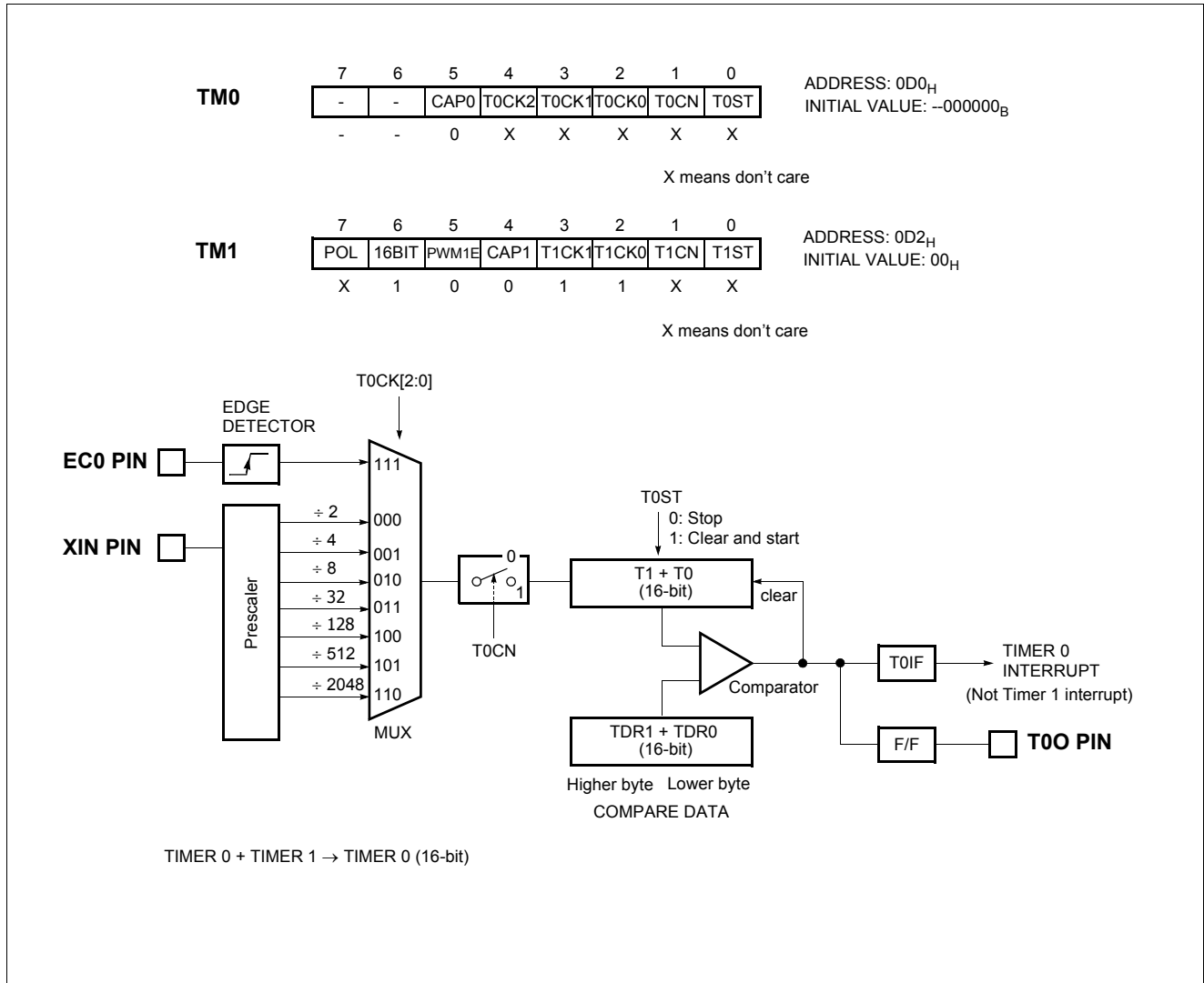
Figure 12-7 16-bit Timer/Counter
