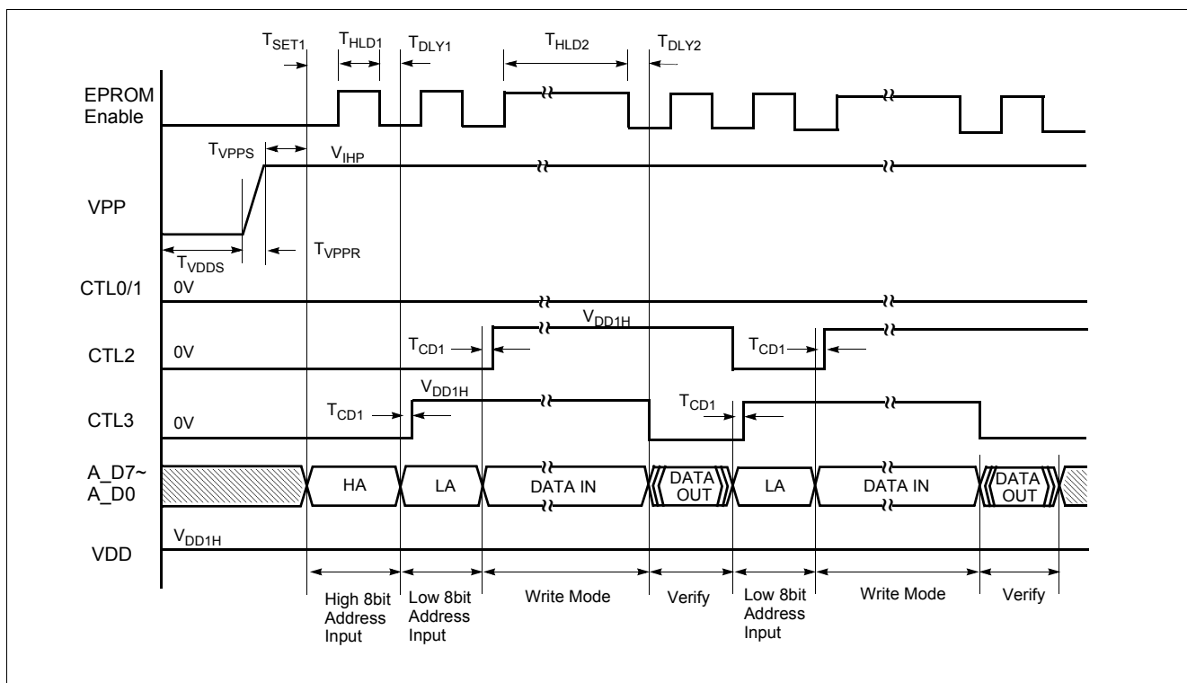
Figure 21-3 Timing Diagram in Program (Write &amp; Verify) Mode
