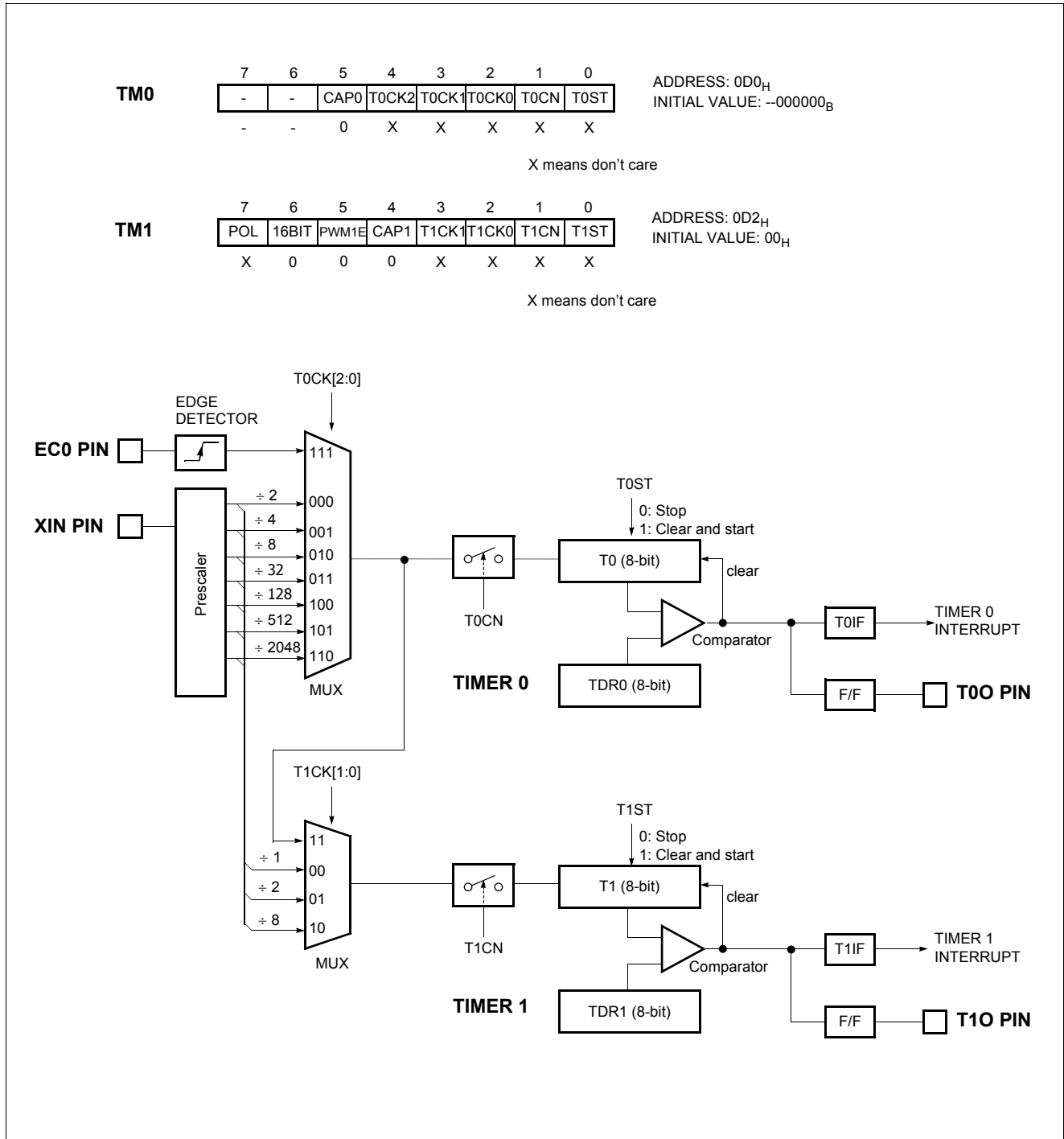
Figure 12-2 8-bit Timer/Counter 0, 1
