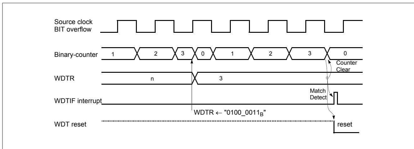
Figure 11-3 Watchdog timer Timing
