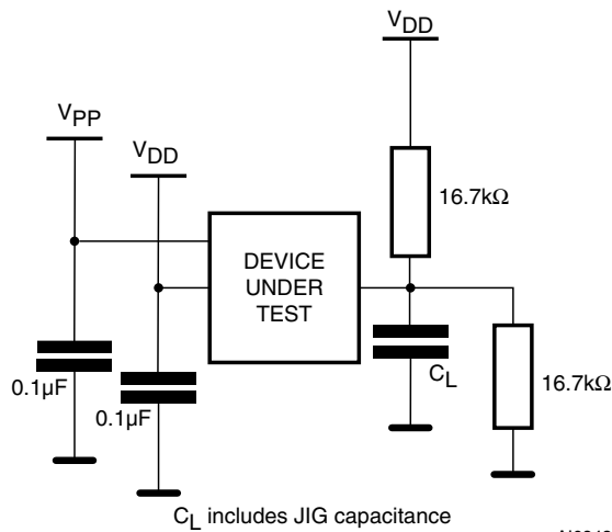
Figure 13. AC Measurement Load Circuit
