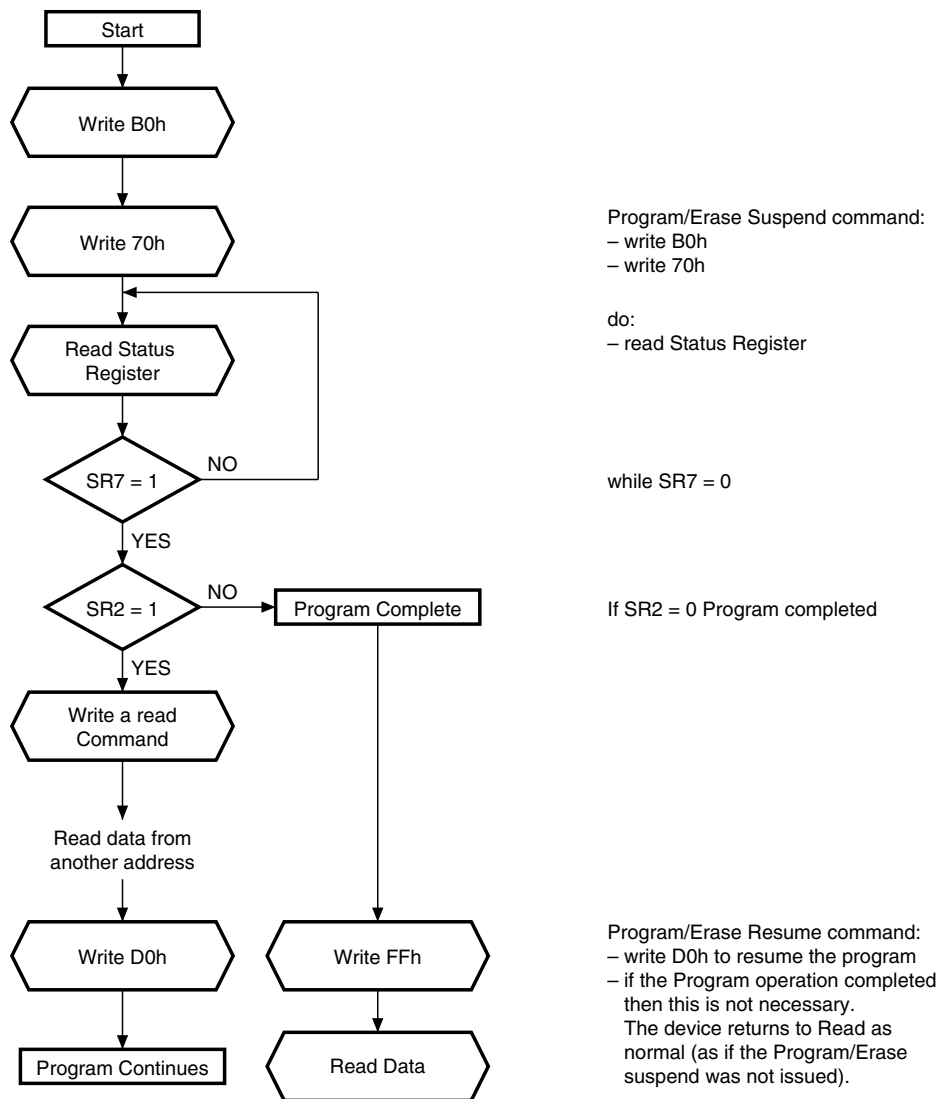
Figure 25. Program Suspend and Resume Flowchart and Pseudo Code
