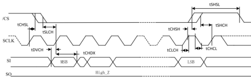
Figure 36. Serial Input Timing
