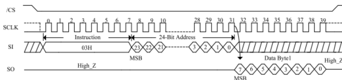
Figure 10. Read Data Bytes Sequence Diagram
