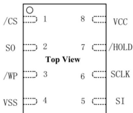
Figure 3. Pin Configuration USON(DFN)4x3mm
