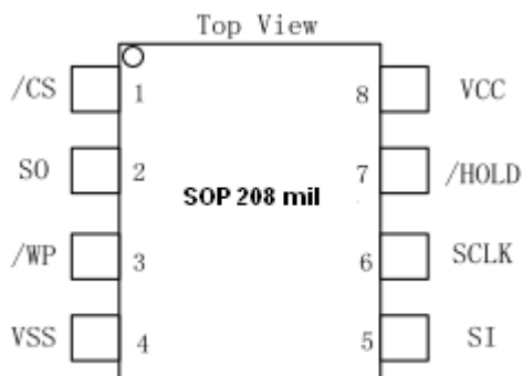
Figure 2. Pin Configuration SOP 208 mil
