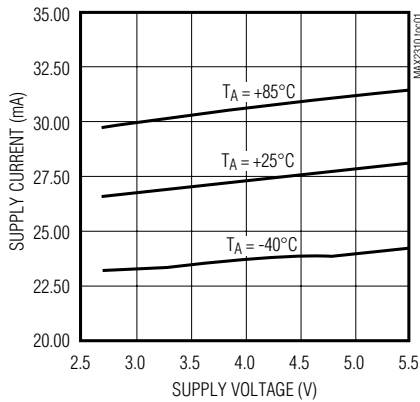
RECEIVE SUPPLY CURRENT vs. SUPPLY VOLTAGE
