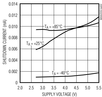
RECEIVE SHUTDOWN CURRENT vs. SUPPLY VOLTAGE
