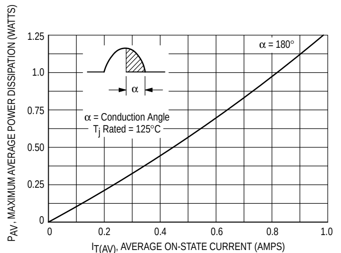
Figure 4. Power Dissipation
