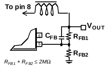
Fig. 4: Adjustable output using ILC6377SO-Adj
