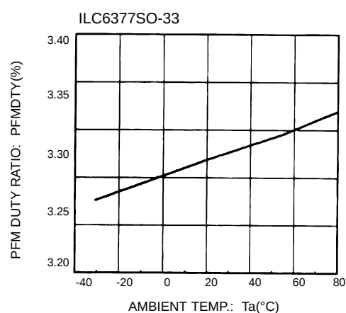
PFM DUTY RATIO vs. AMBIENT TEMPERATURE
