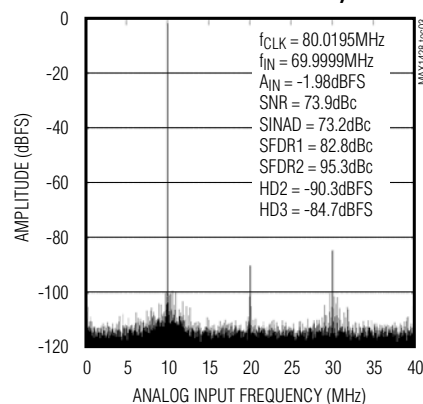
FFT PLOT (32,768-POINT DATA RECORD, COHERENT SAMPLING)
