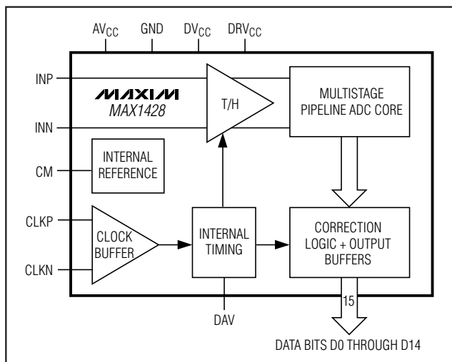
Figure 1. Simplified MAX1428 Diagram
