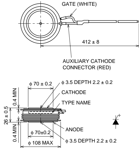
OUTLINE DRAWING
