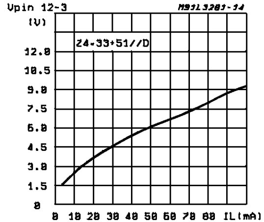
Figure 7: Zener Equivalent.
