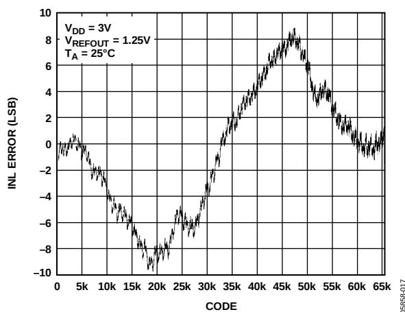
Figure 16. INL—AD5663R-3
