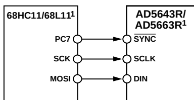
Figure 57. AD5623R/AD5643R/AD5663R to 68HC11/68L11 Interface
