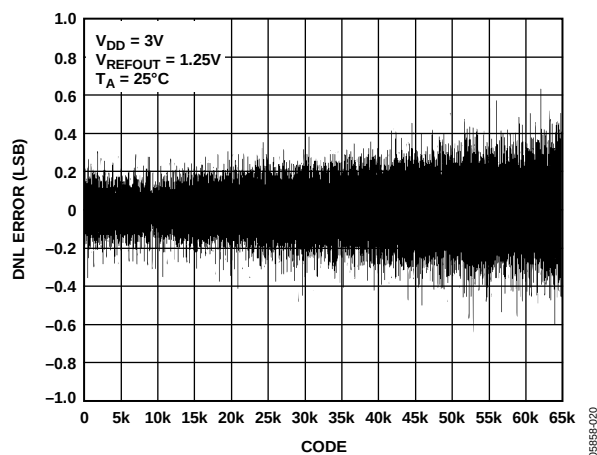
Figure 19. DNL—AD5663R-3
