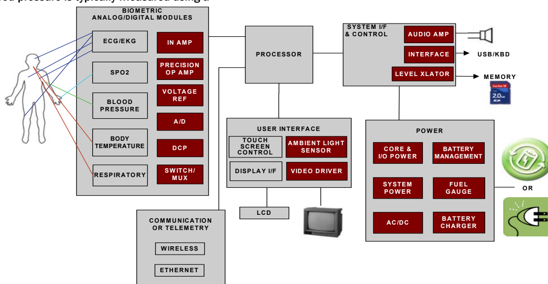
FIGURE 1. BLOCK DIAGRAM OF A PATIENT MONITOR
