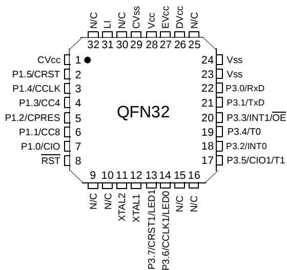
Figure 3. QFN32 Pinout
