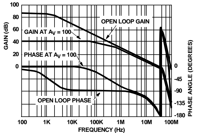
FIGURE 15. FREQUENCY RESPONSE
