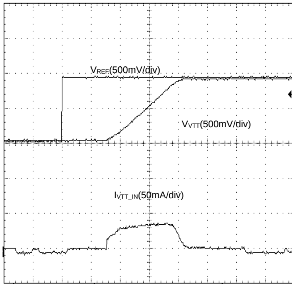
Figure 8. Soft Start
