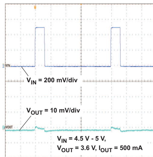
Figure 20. Line Transient
