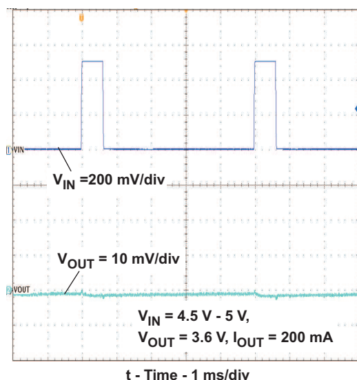
Figure 19. Line Transient
