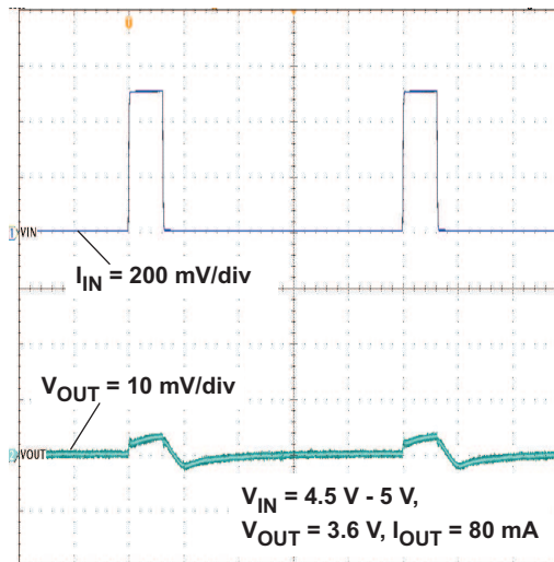
Figure 18. Line Transient
