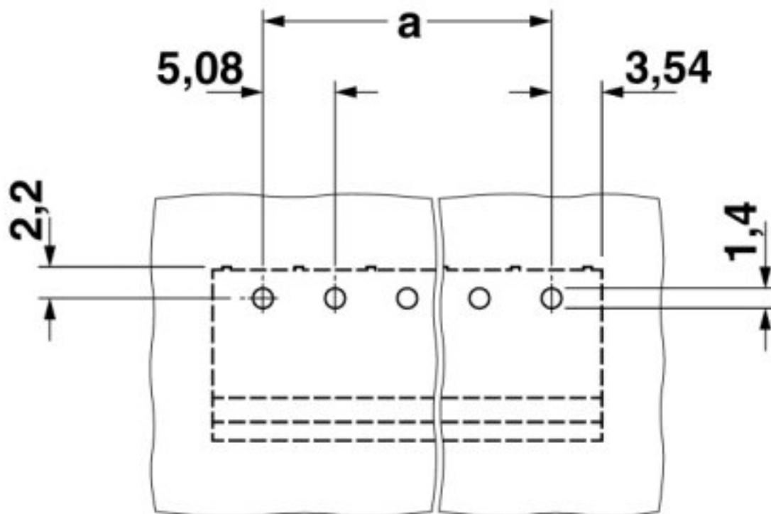
Drilling diagram
