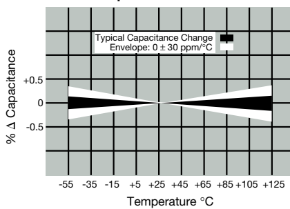
Temperature Coefficient
