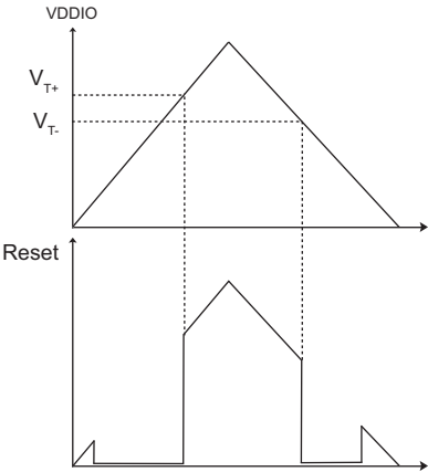
Figure 44-3. Zero-Power-on Reset Characteristics
