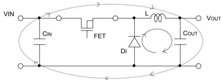
2 Current loop in Buck regulator system
