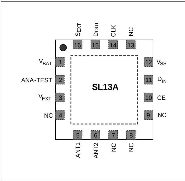
Figure 4: Die Pad Layout
