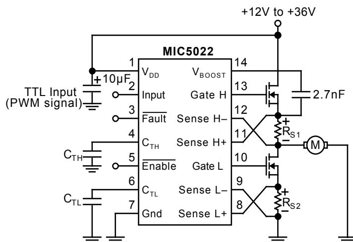
DC Motor Control Application
