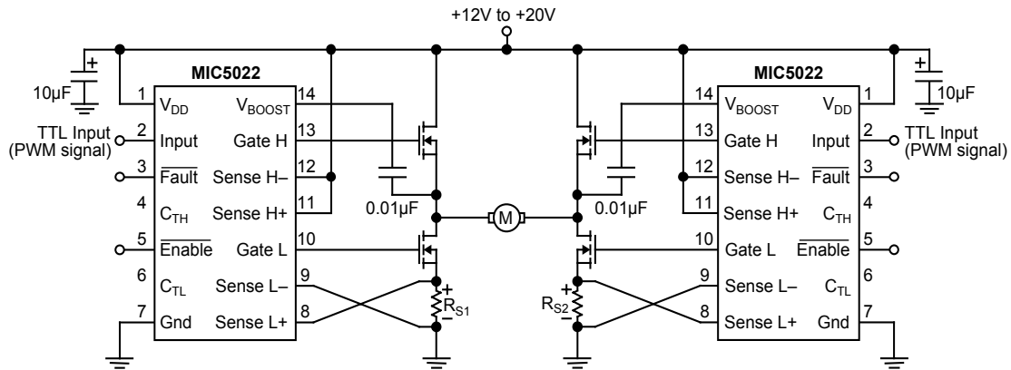
Figure 2. Full-Bridge Motor Control Application
