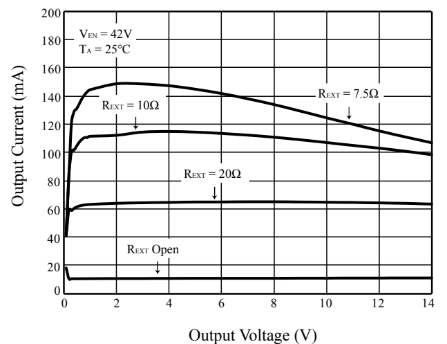
Figure 7 I_{OUT} vs. V_{OUT}
