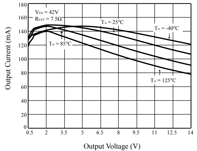
Figure 5 I_{OUT} vs. V_{OUT}
