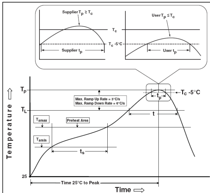
Figure 37 Classification Profile
