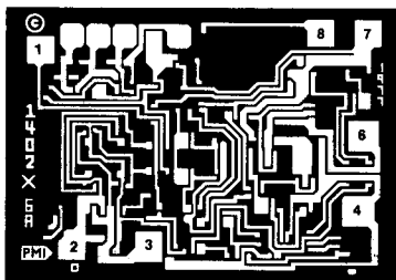
DIE SIZE 0.059 \times 0.043 inch, 2537 sq. mils ( 1.50 \times 1.09 mm, 1.64 sq. mm)
