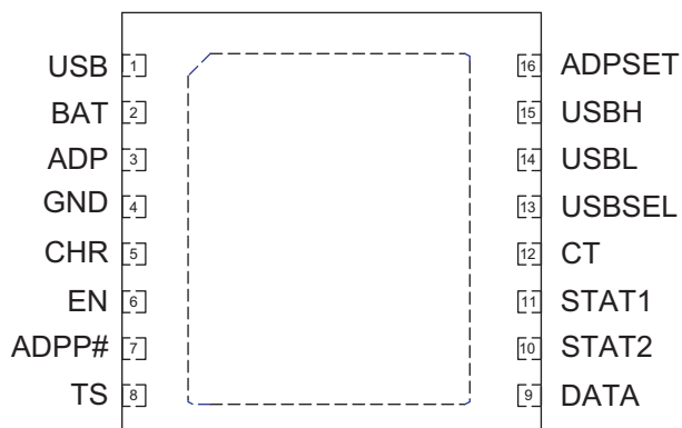
TDFN44-16 (Top View)
