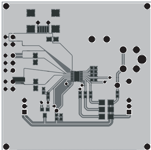
Figure 5: AAT3686 Evaluation Board Component Side Layout.
