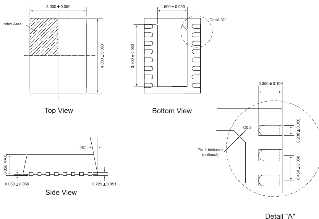
TDFN34-16
