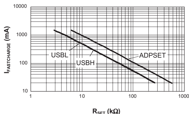
Figure 3: I_{\text{FASTCHARGE}} vs. R_{\text{SET}}
