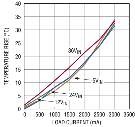
Temperature Rise vs Load Current, 2.5\text{V}_{\text{OUT}}
