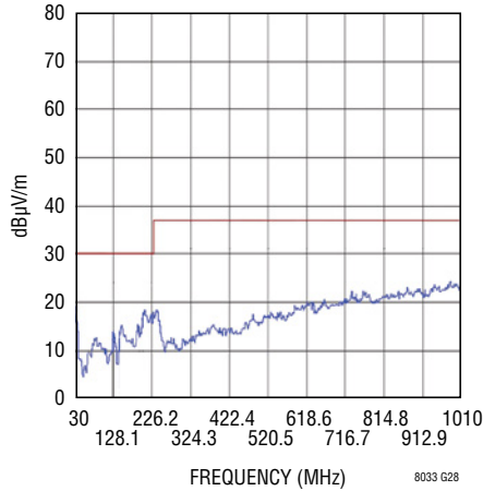
Radiated Emissions, 36\text{V}_{\text{IN}} , 1.2\text{V}_{\text{OUT}} at 3A Load
