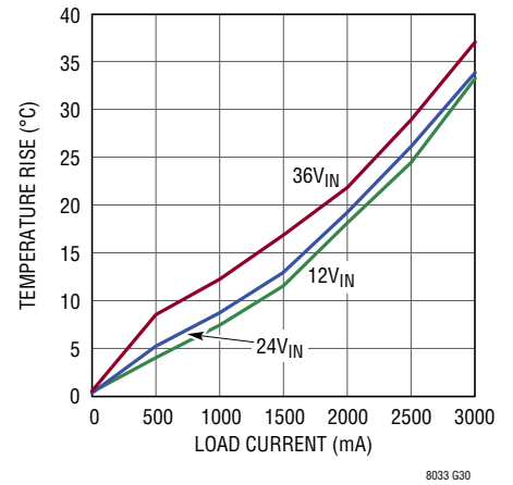
Temperature Rise vs Load Current, 3.3\text{V}_{\text{OUT}}
