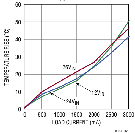
Temperature Rise vs Load Current, 8\text{V}_{\text{OUT}}
