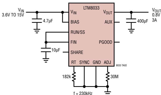
0.8V Step-Down Converter
