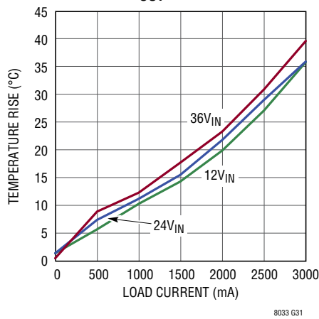
Temperature Rise vs Load Current, 5\text{V}_{\text{OUT}}
