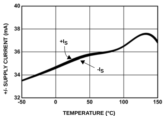
FIGURE 26. +/- SUPPLY CURRENT vs TEMPERATURE
