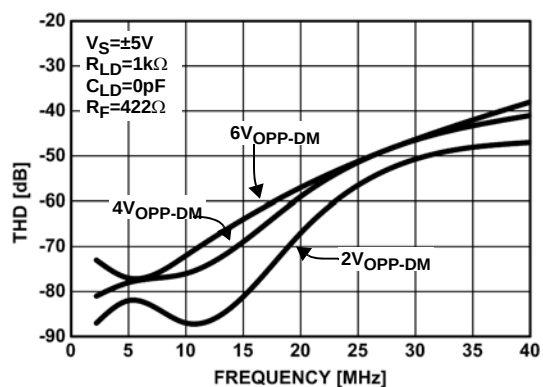
FIGURE 18. TOTAL HARMONIC DISTORTION vs FREQUENCY
