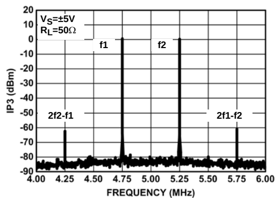
FIGURE 24. THIRD ORDER INTERCEPT POINT
