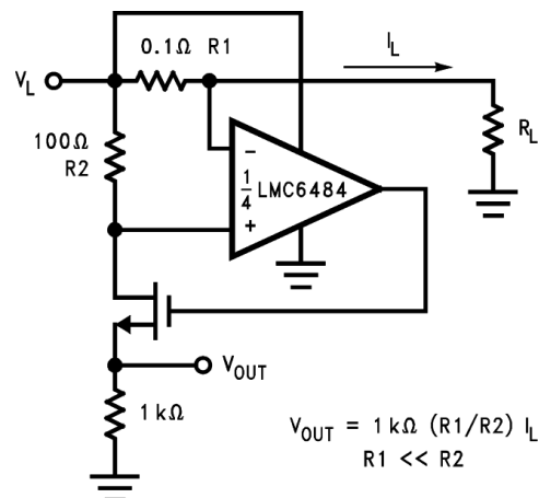
Figure 69. Positive Supply Current Sense
