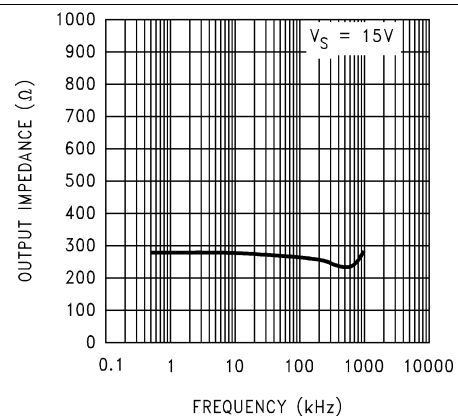
Figure 61. Open Loop Output Impedance vs Frequency
