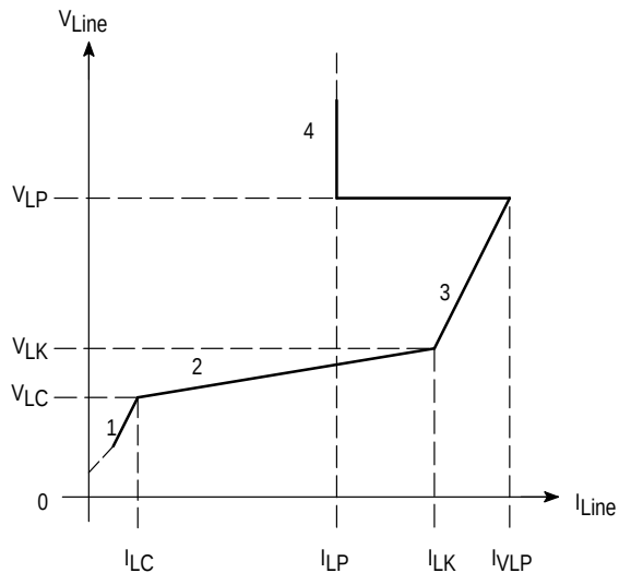
Figure 3. General Form of the DC Mask of the TCA3388
