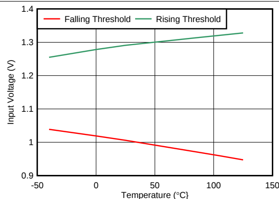
Figure 38. Input UVLOx Threshold vs Temperature
