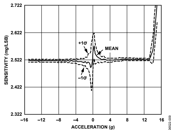
Figure 27. Accelerometer Linearity
