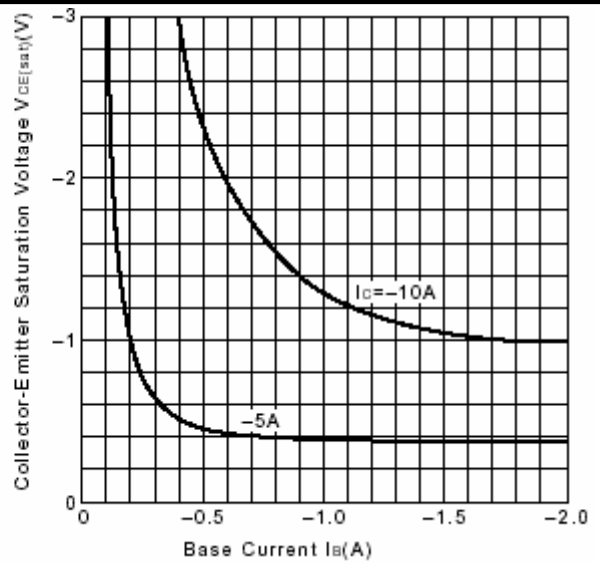
Fig.4 V_{CE(sat)}-I_B Characteristics
