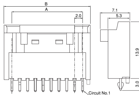
(10 to 12, 15 circuits)
