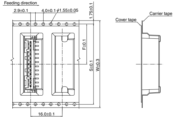
(6 to 12 circuits)
