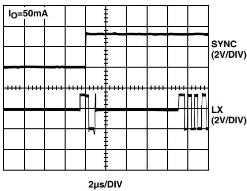
FIGURE 23. PFM-PWM TRANSITION TIME
