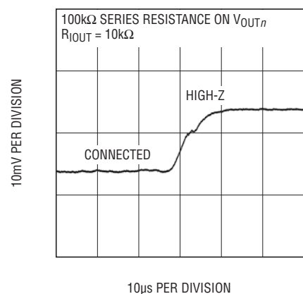
Voltage Buffered IDAC Transient Response During Transition from On State to High-Z State
