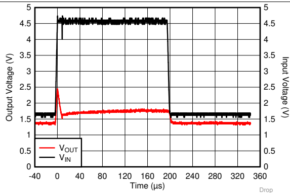
Figure 25. V_{IN} Transient From 1.5 V to 4.5 V
