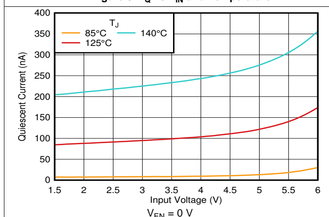
Figure 11. I_{SHDN} vs V_{IN} and Temperature
