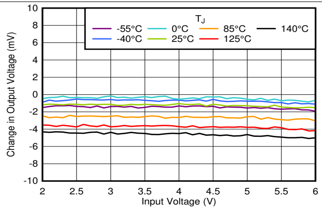
Figure 26. Line Regulation vs V_{IN} and Temperature
