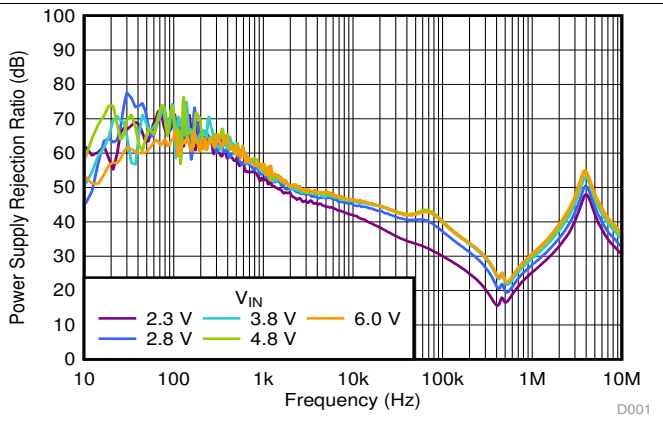
Figure 46. PSRR vs Frequency and V_{IN}
