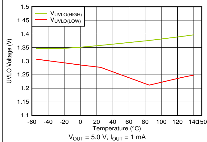
Figure 41. UVLO Rising and Falling Threshold vs Temperature
