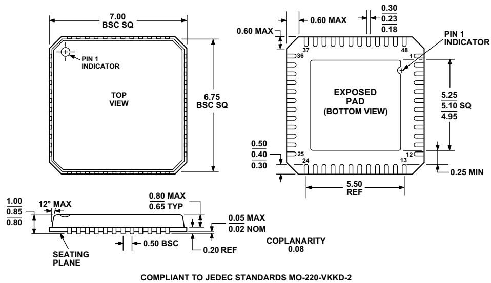
Figure 6. 48-Lead Lead Frame Chip Scale Package [LFCSP_VQ] 7 mm x 7 mm Body, Very Thin Quad (CP-48-1) Dimensions shown in millimeters
